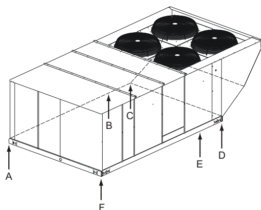
ZW/ZK Unit 6 Point Load Weight
